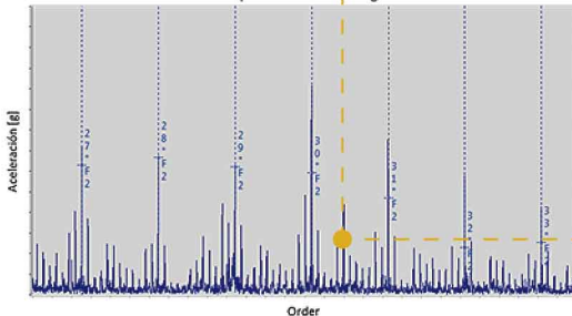
Espectro Order Tracking
